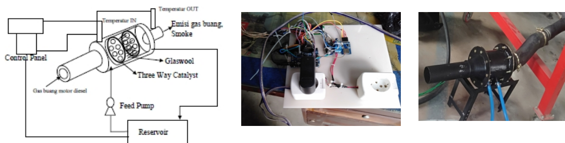
Figure 3. Catalytic Conveter (CAT) Diesel Design
