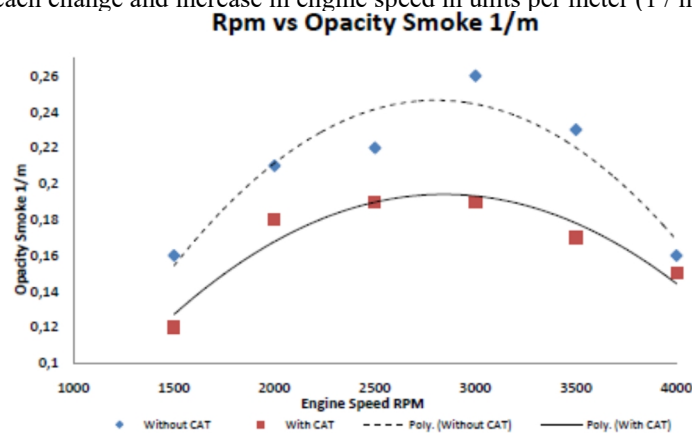
Figure 6. Graph of Opacity (1 / m) at various engine speed (Rpm)
