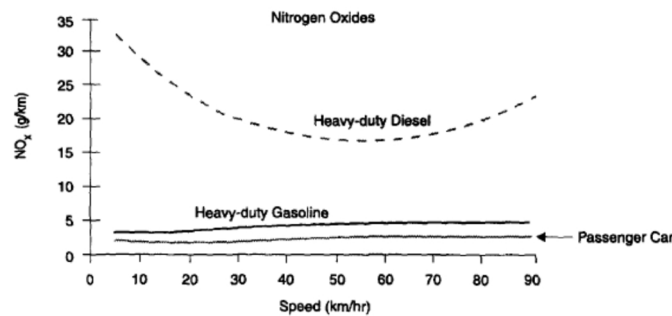
Figure 1. Diesel Motor NO x Graph (Faiz, 1996)
