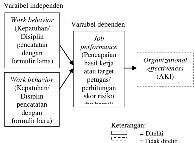
Gambar 1. Variabel Independen
